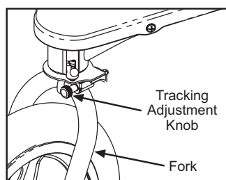
Fig. 13 Tracking Adjustment.
